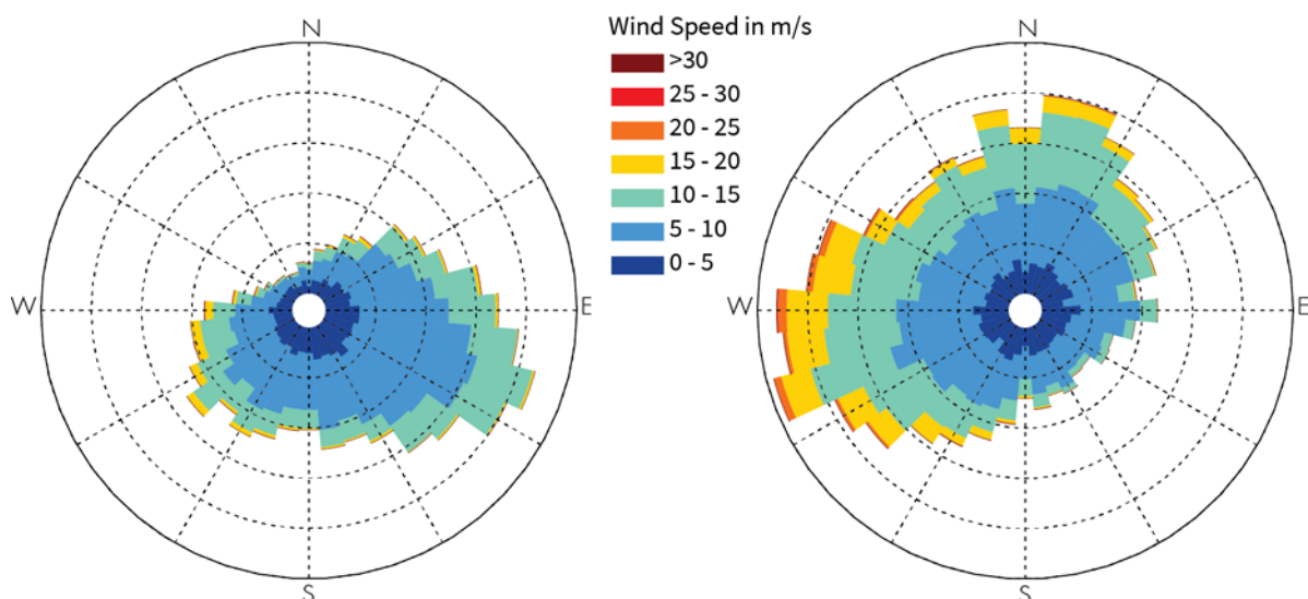
Figure 3: Modelled wind speed and direction roses for summer (left) and winter (right) at 35°S, 130°E for the period 1994-2014 (NCEP/NCAR global reanalysis).
